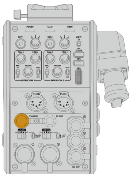
Tracker Interface connector
